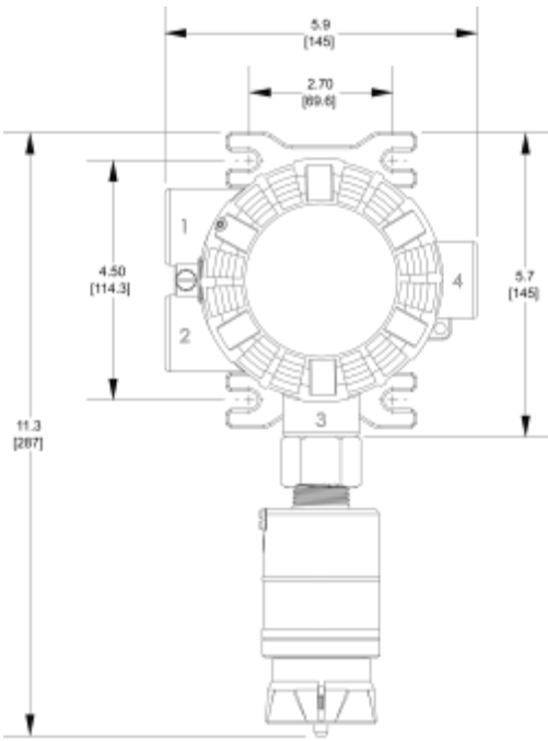
Figure 50 ULTIMA X5000 Height & Width with M25 Adapter
