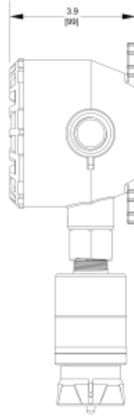
Figure 51 Short Lid Depth with M25 Adapter
