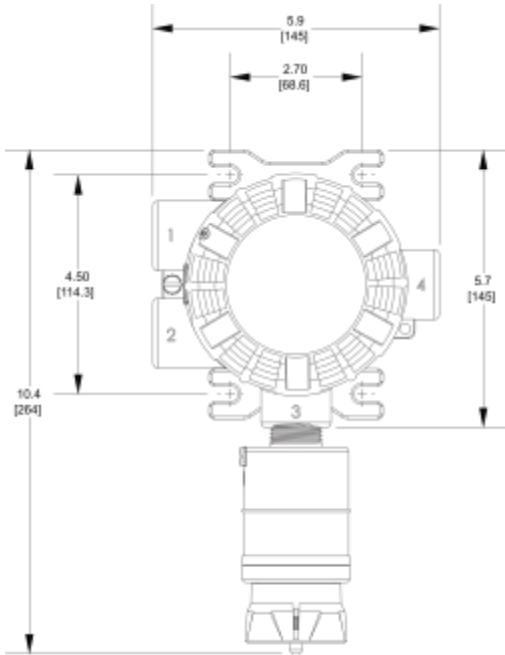
Figure 46 ULTIMA X5000 Height & Width
