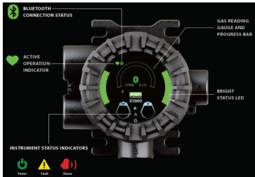
Figure 1 OLED Display
