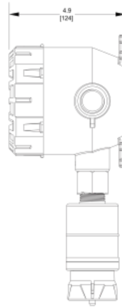
Figure 52 Deep Lid Depth with M25 Adapter
